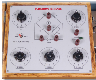
Schering Bridge
