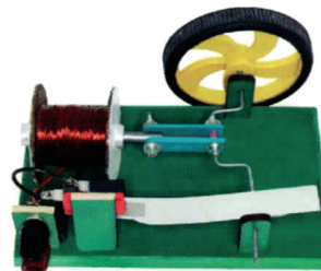
Solnoid Engine
