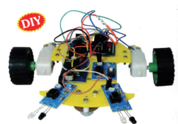
Sound and LDR Based Robo Car
